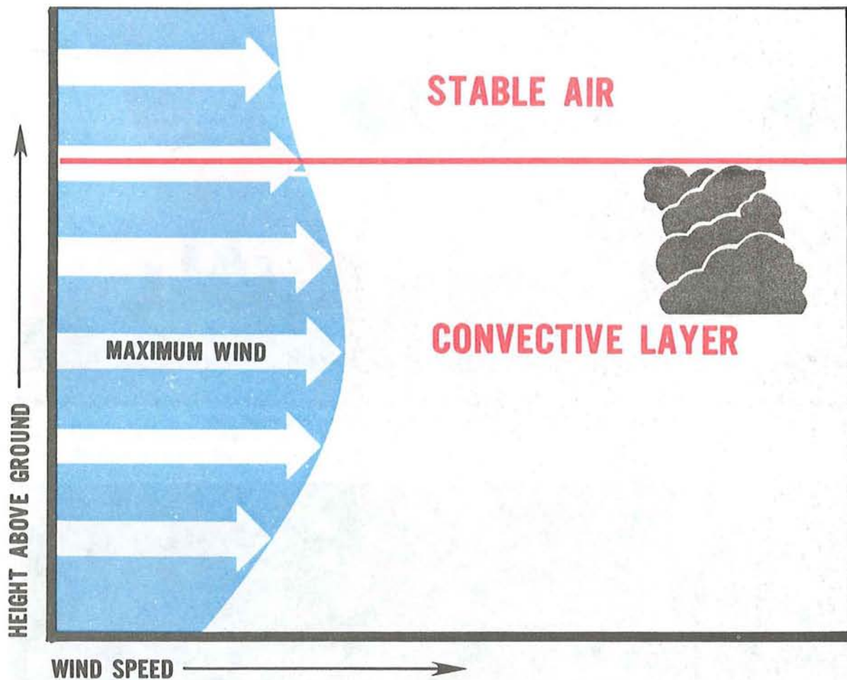
FIGURE 158. Conditions favorable for thermal strecting. A very stable layer caps the convective layer, and wind reaches a maximum within the convective layer. If cumulus clouds mark thermal streets, the top of the convective layer is about the height of the cloud tops.
