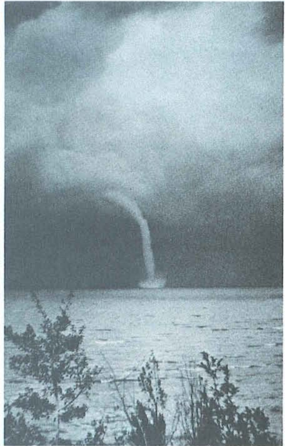
FIGURE 108. A waterspout.
