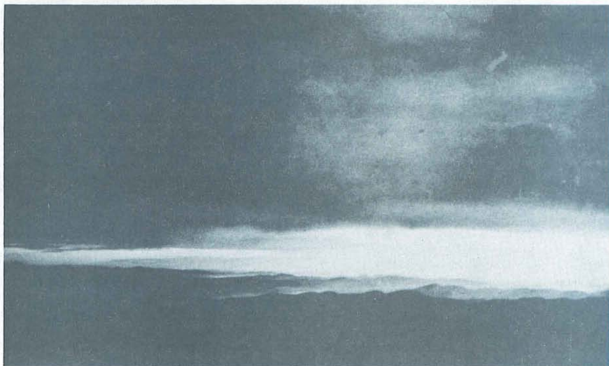
FIGURE 49. ALTOSTRATUS. Altostratus is a bluish veil or layer of clouds. It is often associated with altocumulus and sometimes gradually merges into cirrostratus. The sun may be dimly visible through it. Little or no turbulence with moderate amounts of ice.
